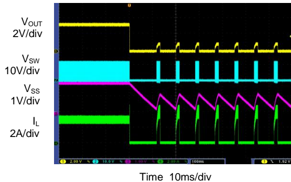
Short Circuit Protection ( I_{OUT}=3\text{A} )
