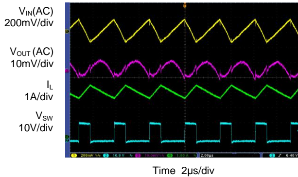
Output Ripple ( I_{OUT}=3\text{A} )
