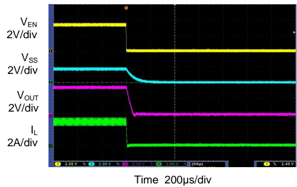
Enable Turn-off Characteristic ( V_{IN}=12\text{V} , V_{EN}=3.3\text{V} , V_{OUT}=3.3\text{V} , I_{OUT}=3\text{A} )
