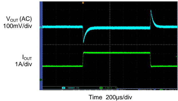
Load Transient ( I_{OUT}=1.5 to 3\text{A} )
