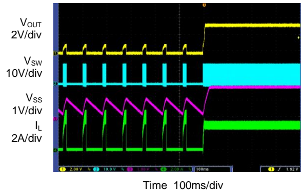
Short Circuit Recovery ( I_{OUT}=3\text{A} )
