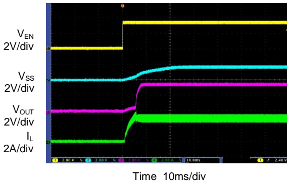
Enable Turn-on Characteristic ( V_{IN}=12\text{V} , V_{EN}=3.3\text{V} , V_{OUT}=3.3\text{V} , I_{OUT}=3\text{A} )
