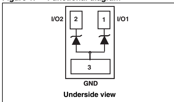
Figure 1. Functional diagram
