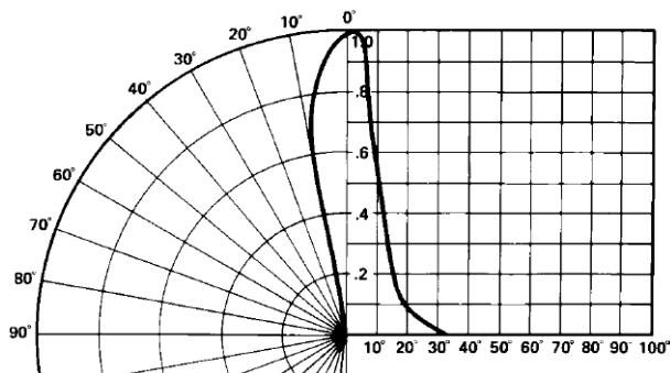
Figure 7: Relative Luminous Intensity vs. Angular Displacement, HLMP-D155
