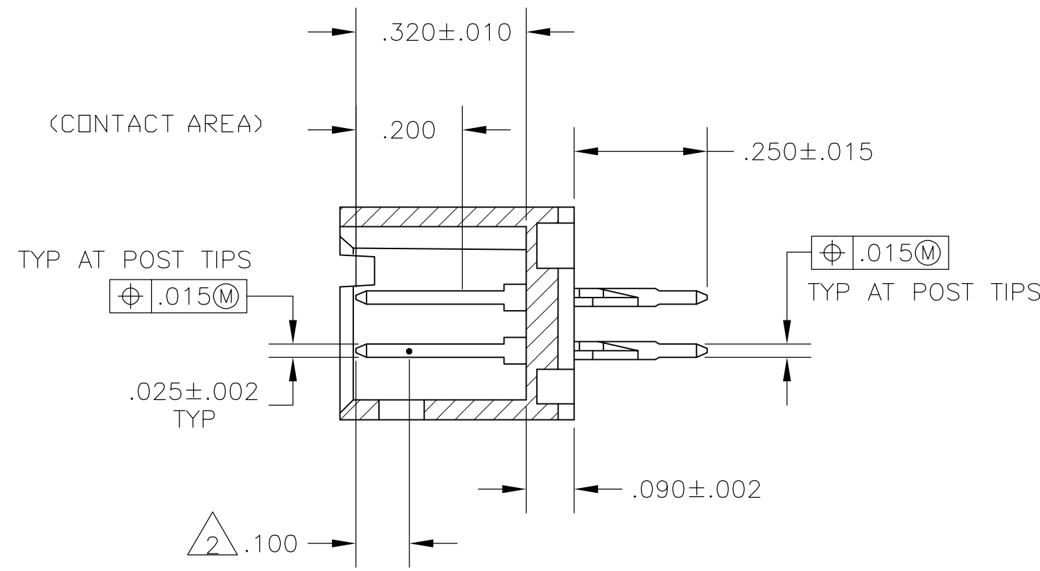
SECTION X-X
