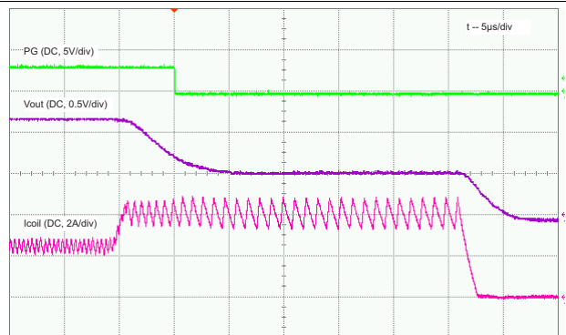
Figure 19. Output Short-Circuit Protection, Load = 0.47 Ω, Entry
