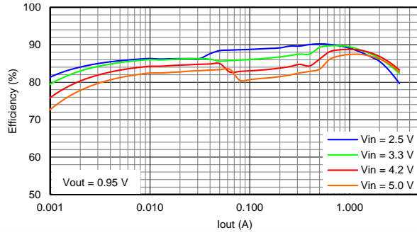
Figure 4. Efficiency
