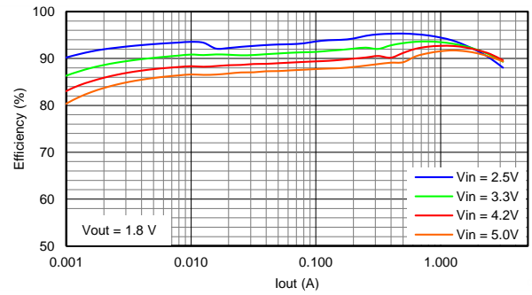
Figure 5. Efficiency
