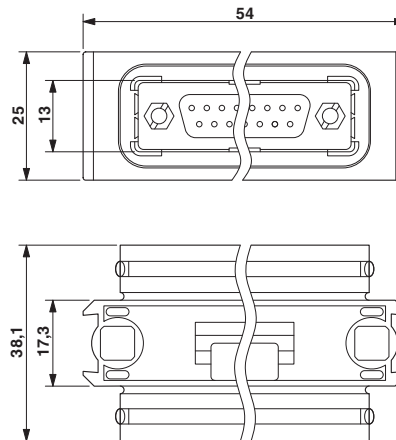
Dimensional drawing
