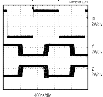
DRIVER PROPAGATION DELAY ( SLO = HIGH )
