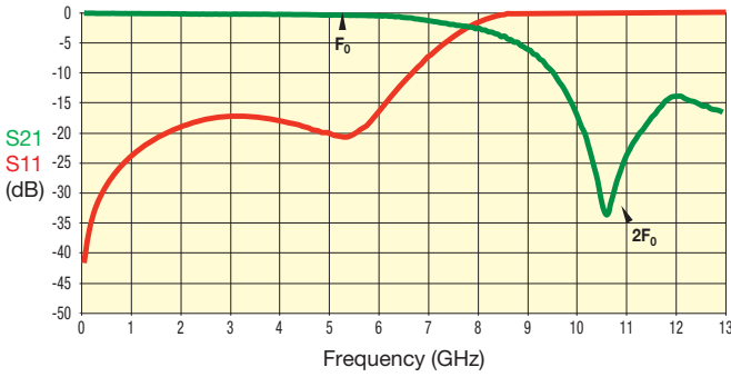
LP0603N5500ANTR
