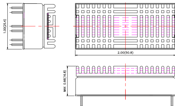
Measurement shown in inches and (millimeters)
