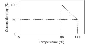
Derating of Rated Current
