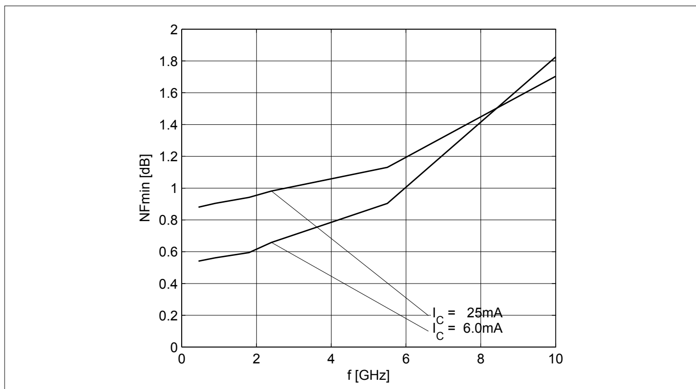
Figure 17 Noise figure NF_{min} = f(f) , V_{CE} = 3 V, Z_S = Z_{S,opt} , I_C = 6 / 25 mA
