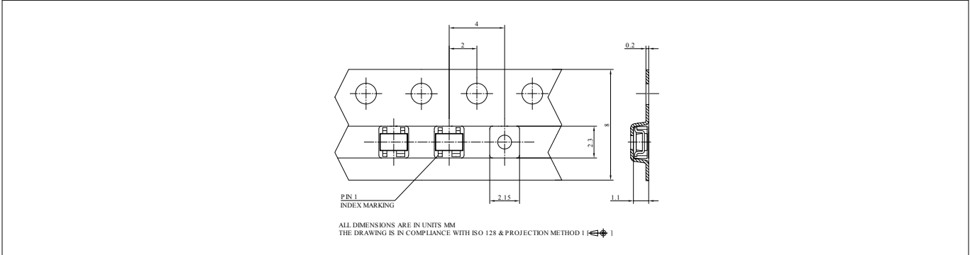
Figure 23 Tape dimensions
