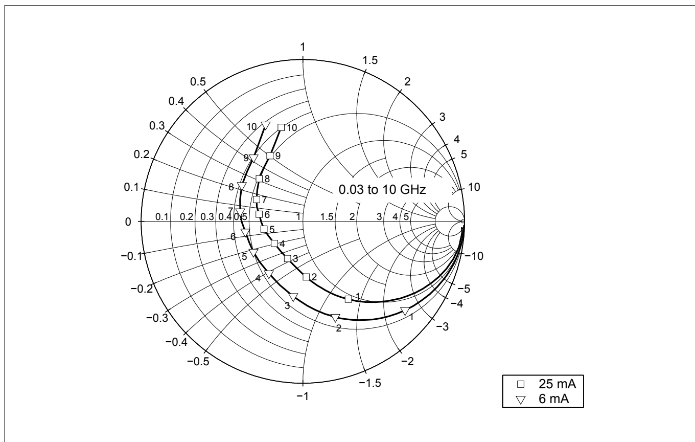
Figure 16 Output reflection coefficient S_{22} = f(f) , V_{CE} = 3 V, I_C = 6 / 25 mA
