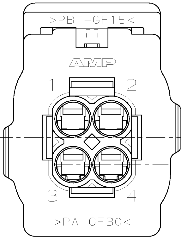
VIEW B-B
