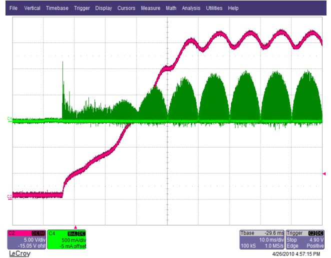
Figure 24 – 265 VAC, Full Load. Upper: I_{RIPPLE} , 0.5 A / div. Lower: V_{OUT} , 5 V, 10 ms / div.
