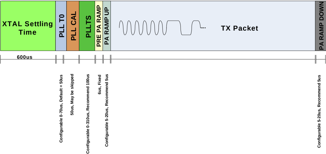
Figure 8. TX Timing
