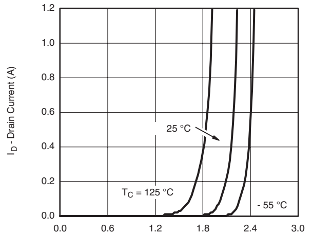
T_C = 125 \text{ }^\circ\text{C} and -55 \text{ }^\circ\text{C} Transfer Characteristics
