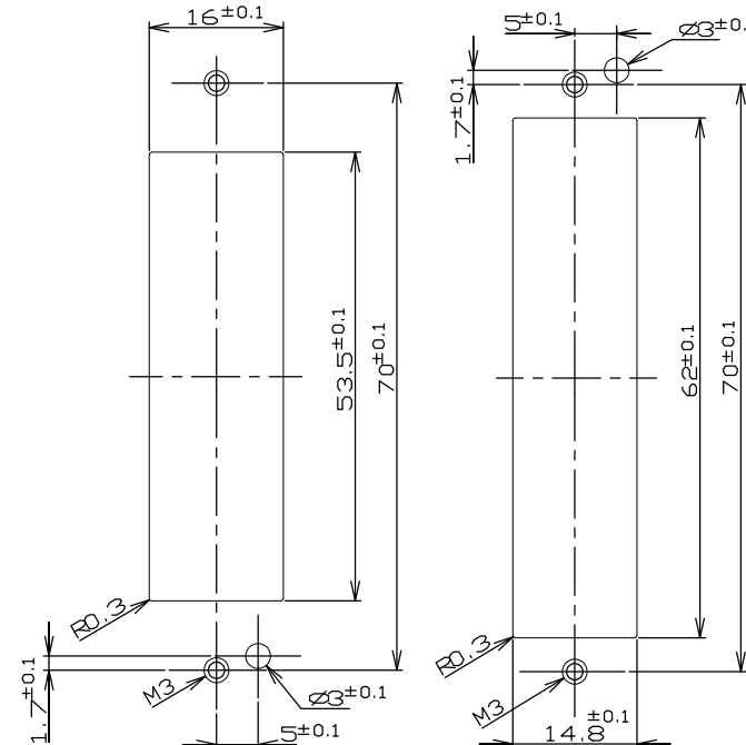
VIEW S PANEL CUT DIMENSIONS (CONNECTOR MATING SIDE)
