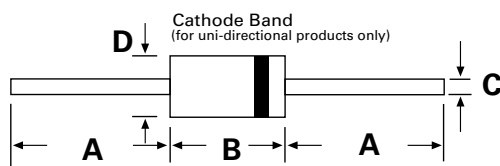
DO-204AC (DO-15)
