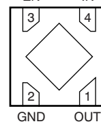
DQN Package 4-Pin X2SON Bottom View
