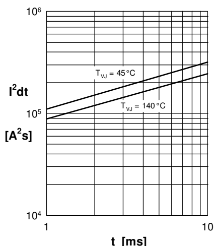
Fig. 2 I^2dt versus time
