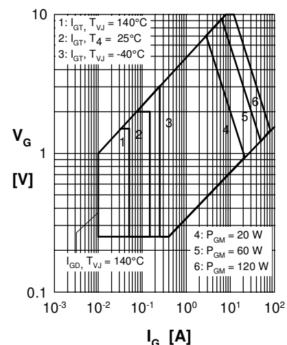
Fig. 5 Gate voltage and current
