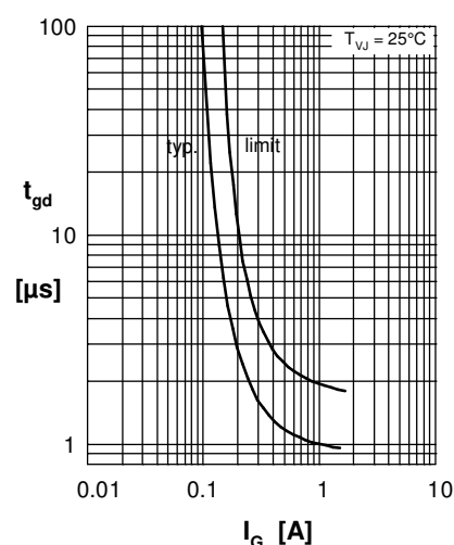
Fig. 7 Gate trigger characteristics
