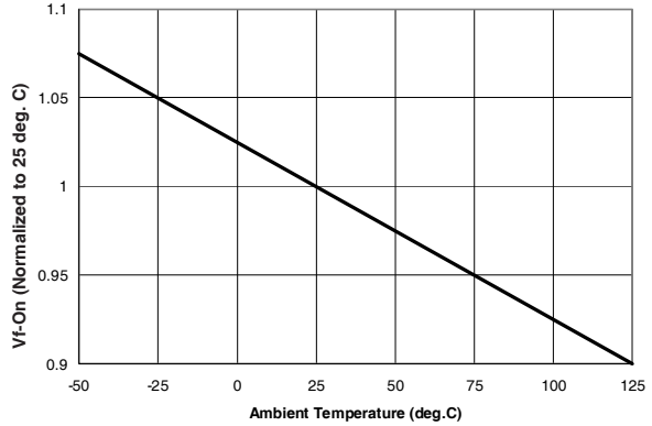
Figure 4. Typical Normalized VCEON
