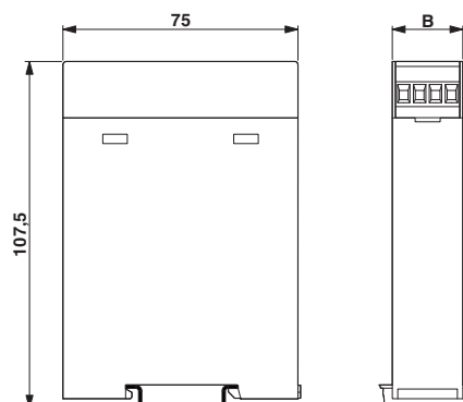
Dimensional drawing
