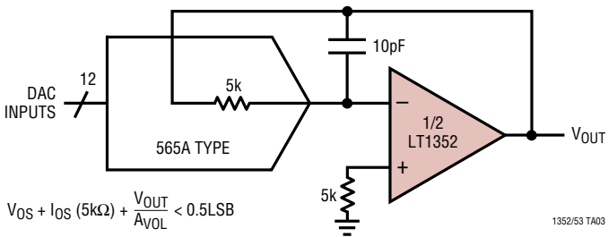
DAC I-to-V Converter
