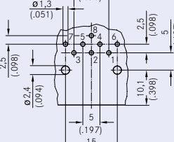
8 POL
