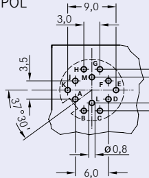
12 POL
