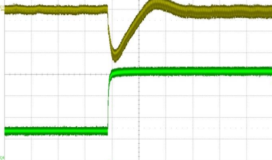
Figure 16 - Load transient V_1 , 20 to 45 A (500 \mu s/div) CH1: V_1 (200 mV/div) CH4: I_1 (10 A/div)
