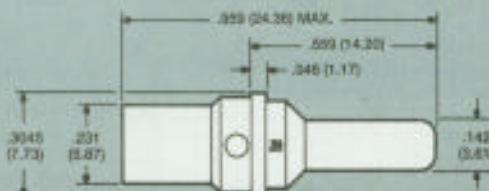
Socket Contact Size 8 LMD-4108-36L
