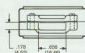
WIRE OUTLET WITH STRAIN RELIEF CLAMP REVERSED
