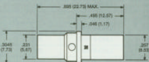
Socket Contact Size 8 LMD-4108-36L
