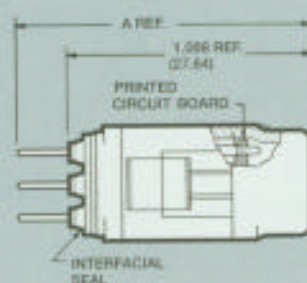
MODULE (SIDE VIEW)
