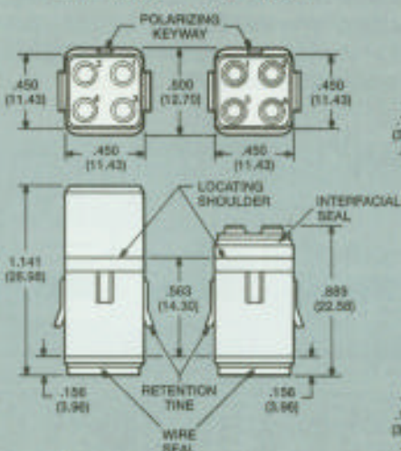
Sealed Socket Module LMD-4005-S
