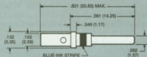
Socket Contact Size 16 LMD-4116-96LD
