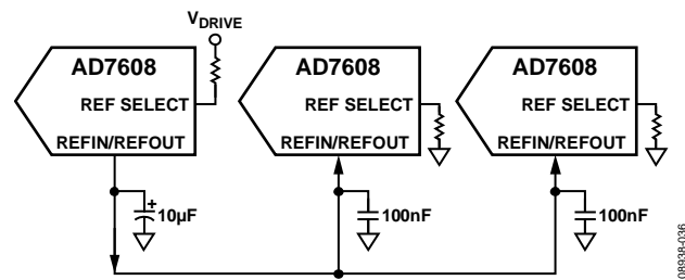
Figure 39. Internal Reference Driving Multiple AD7608 REFIN Pins
