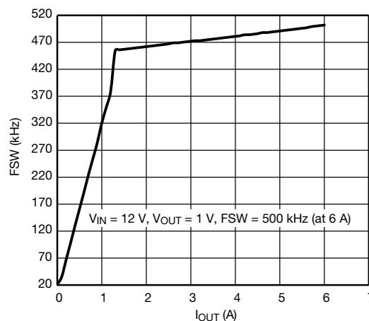
f_{SW} vs. I_{OUT} (in Power-Save-Mode)
