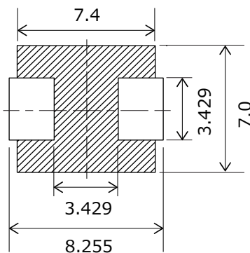
Series PCC-M0630M-LP (ETQP3M□□□KVN)
