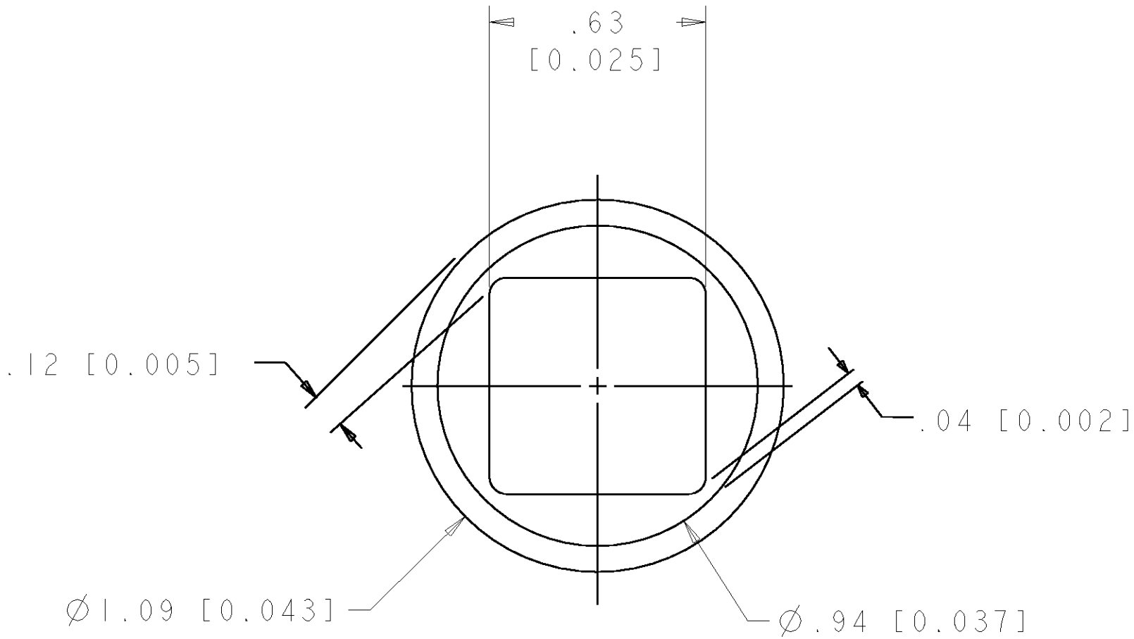
SOLDER TERMINATION AREA SCALE 40:1 RECOMMENDED PRINTED CIRCUIT SOLDER HOLE FINISHED HOLE: Ø1.02 [.040] ±.008 [.0003] DRILLED HOLE: Ø1.15 [.0453] ±.013 [.0005] COPPER PLATE: .025 [.0010] MIN TIN PLATE: .008 [.0003] MIN. (PER SURFACE)
