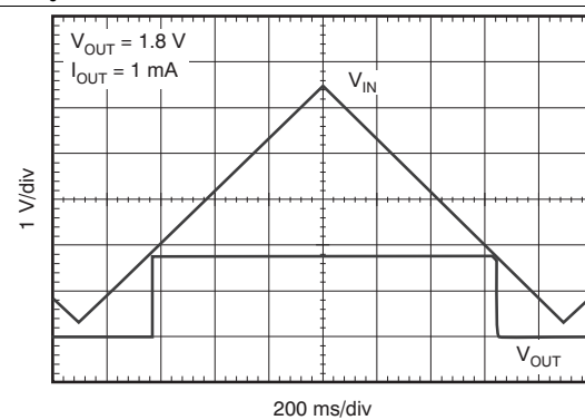
Figure 20. V_{IN} Ramp Up, Ramp Down Response
