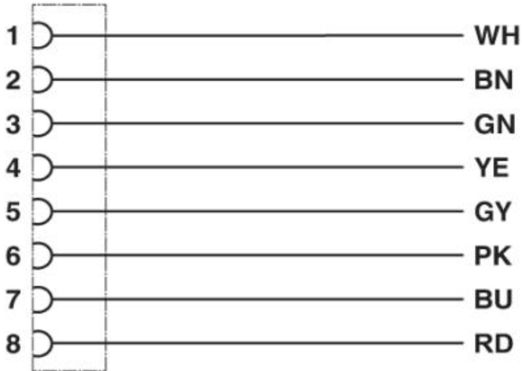
Contact assignment of M8 socket
