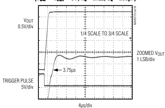
MAJOR CODE TRANSITION GLITCH ENERGY ( V_{DD} = V_{REF} = 5\text{V} , R_L = 2\text{k}\Omega , C_L = 200\text{pF} )
