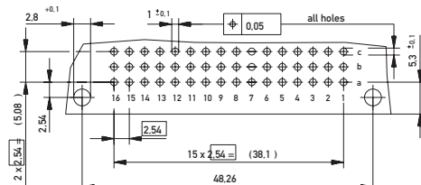
PCB drillhole pattern
