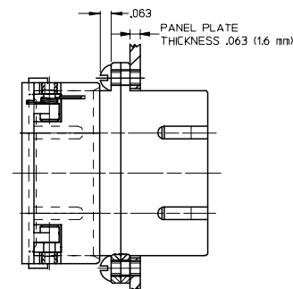
RECOMMENDED MOUNTING VERSION 2
