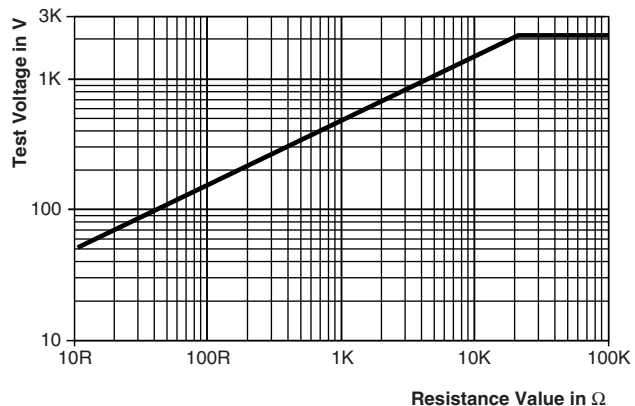
10 / 700 Pulse
