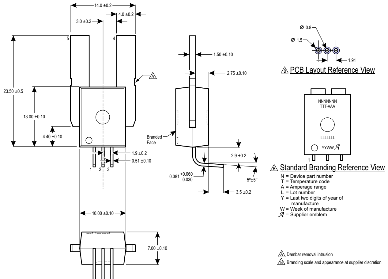
Package CB, 5-pin Package, Leadform PSF
