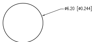
PANEL CUTOUT
