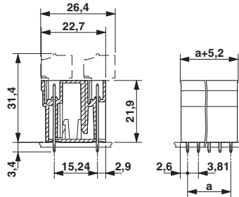
Dimensional drawing
