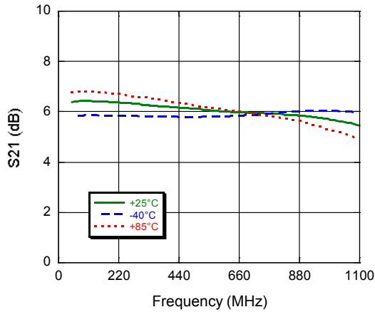
Gain - OUT3
