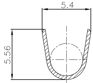
SECT "C-C"
