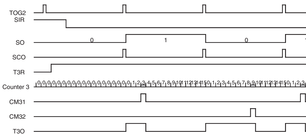
Figure 24-9. Pulse-width Modulation
