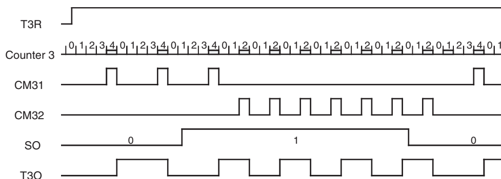
Figure 24-8. FSK Modulation
