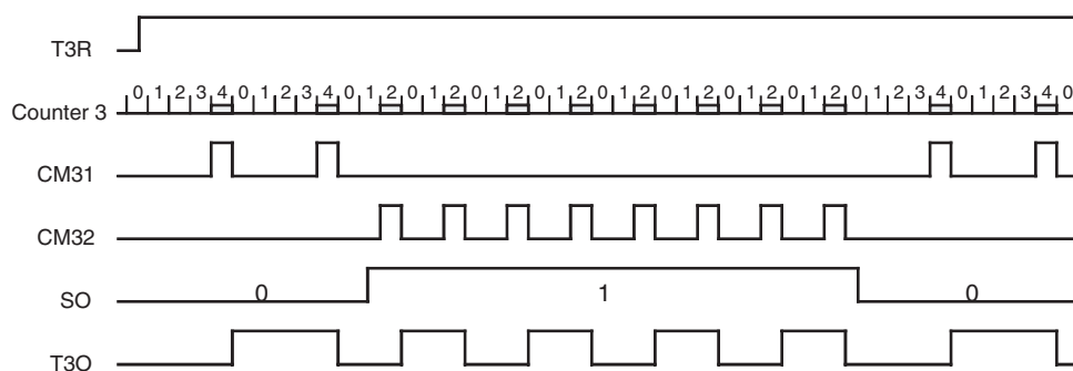
Figure 24-18. FSK Modulation
