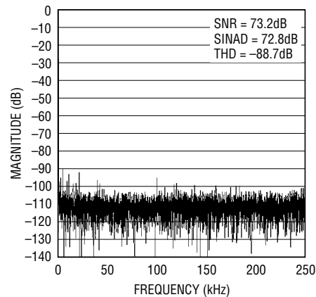
Figure 4. 1kHz Sine Wave 8192 Point FFT Plot (LTC2306)
