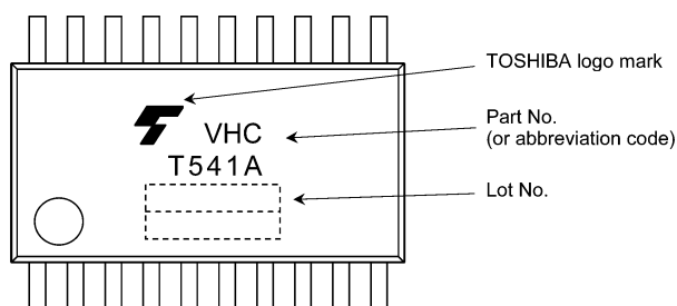
74VHCT541AFT
