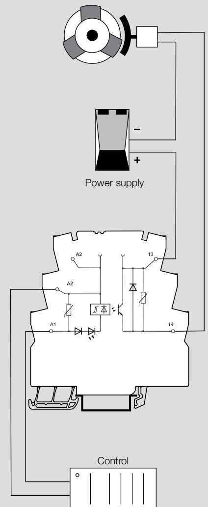
Example: motor brake
