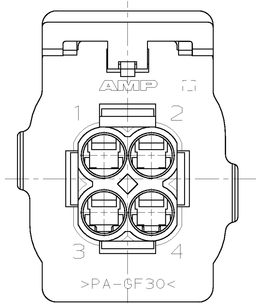
VIEW B-B
