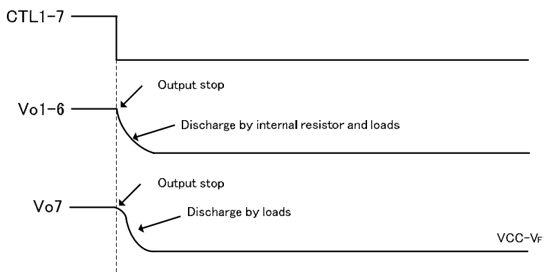
Fig. 6 stop sequence
