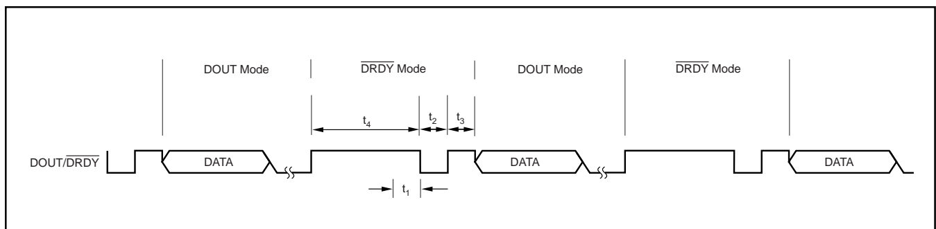
FIGURE 12. DOUT/DRDY Partitioning.
