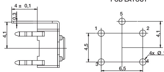
PCB LAYOUT
