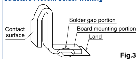
Structure Prevent Solder Wicking
