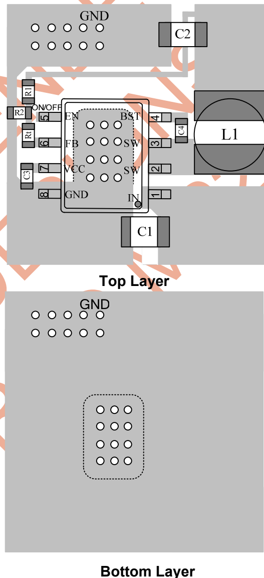
Figure 4—PCB Layout
